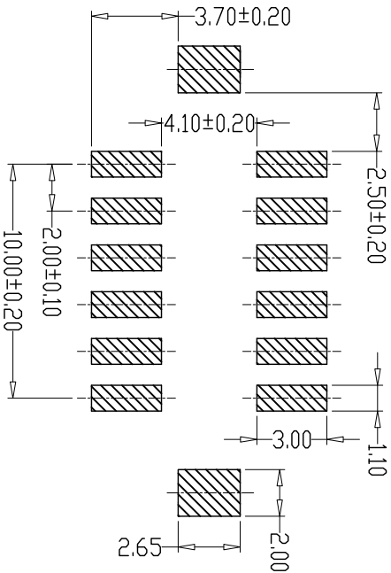
PCB LAYOUT
